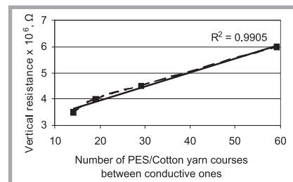
Figure 5. Vertical resistance of knitted fabrics with conductive S-Shield PES yarns after 5 washing cycles (Control fabric: after 5 washing cycles R = 1.64 \times 10^8 \Omega ).
